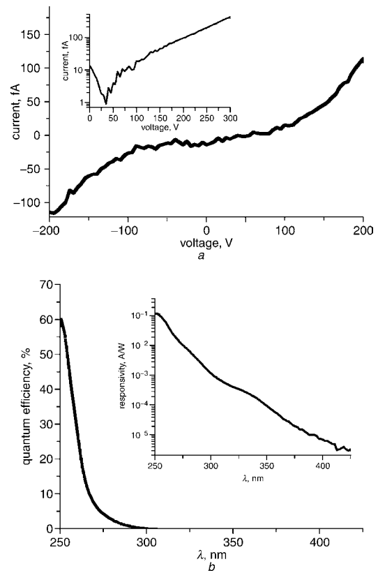
Fig. 2 I–V measurement of an \text{Al}_{0.6}\text{Ga}_{0.4}\text{N} MSM photodiode
