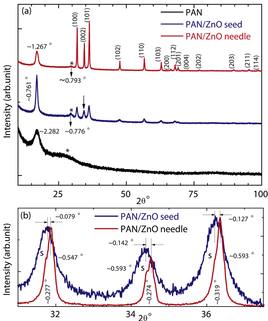
Fig. 4. (a) XRD patterns of nanofibers of PAN, PAN/ZnO seed and PAN/ZnO needle, and (b) magnified XRD patterns in the range of 31–37.5°.
